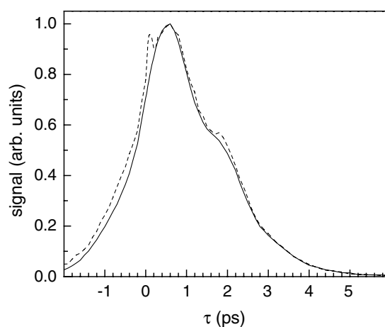
Fig. 4. Comparison of the vibrational echo decays for high concentration (solid line) and low concentration (dashed line) solutions at 1951\text{ cm}^{-1} , demonstrating that the Hb–CO dynamics in aqueous solution are insensitive to the effects of concentration and viscosity.
