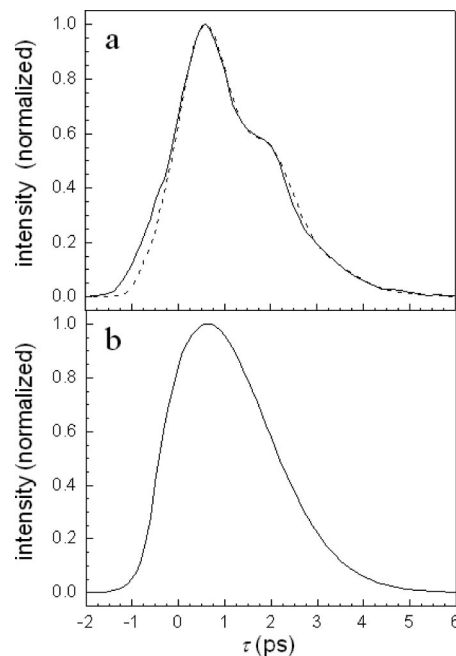
FIG. 6. (a) Hb–CO data at high intensity detected at the 0-1 transition frequency (solid curve) and the corresponding third order calculation which includes both the main absorption band and the blueshifted substate band. The data are accurately reproduced by the strictly third order calculation. (b) The same third order calculation without the inclusion of the blueshifted substate band. The lack of beats demonstrates that the ADB mechanism is responsible for the beats.
