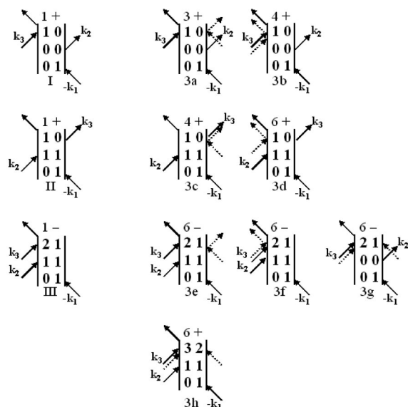
FIG. 8. Third order diagrams giving rise to the vibrational echo signal and the related fifth order diagrams with the two additional radiation field-matter interactions occurring in pulse 3 ( \pm k_3 ). The coherence periods caused by the extra interactions are omitted, but the population periods are shown explicitly. The two additional interactions are shown as dashed arrows. The number of permutations of the incoming fields and the sign of the diagram are shown before each diagram.
