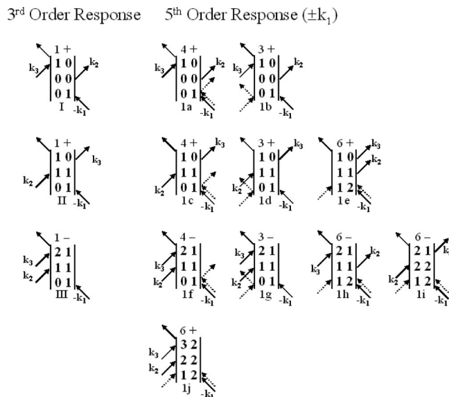
FIG. 4. Third order diagrams giving rise to the vibrational echo signal and the related fifth order diagrams with the two additional radiation field-matter interactions occurring in pulse 1 ( \pm k_1 ). The coherence periods caused by the extra interactions are omitted, but the population periods are shown explicitly. The two additional interactions are shown as dashed arrows. Diagram 1e causes oscillations in the vibrational echo decays at the 0-1 transition frequency. Diagrams 1h and 1i cause oscillations in the vibrational echo decays at the 1-2 transition frequency. The number of permutations of the incoming fields and the sign of the diagram are shown before each diagram.
