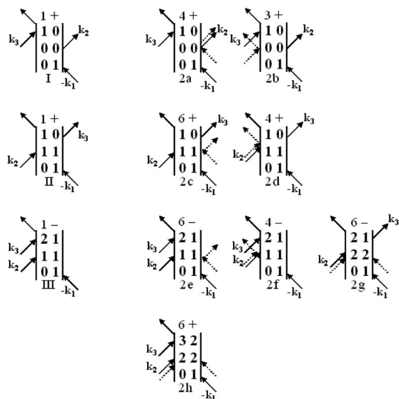
FIG. 7. Third order diagrams giving rise to the vibrational echo signal and the related fifth order diagrams with the two additional radiation field-matter interactions occurring in pulse 2 ( \pm k_2 ). The coherence periods caused by the extra interactions are omitted, but the population periods are shown explicitly. The two additional interactions are shown as dashed arrows. The number of permutations of the incoming fields and the sign of the diagram are shown before each diagram.
