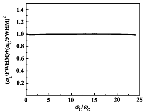
FIG. 7. Equation (A1) is plotted as a function of \omega_L/\omega_G . The almost constant value of 1 demonstrates the validity of the approximation used to obtain the homogeneous contribution and the absolute amplitudes of the FFCF using the simple CLS and linewidth methods.
