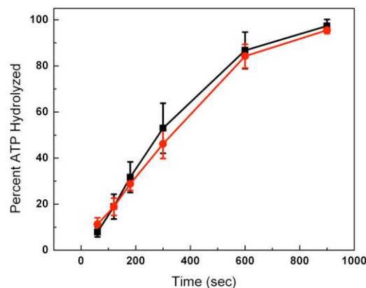
Fig. S3. ATPase activity of QD-tagged FtsK. ATP hydrolysis reactions were conducted at room temperature in buffer containing 40 mM Tris (pH 8), 0.2 mg/mL BSA, 1 mM DTT, 50 mM NaCl, 2 mM MgCl_2 , 1 nM lambda phage DNA, 1 mM ATP, and 100 pM FtsK trimer. Reactions were terminated at the indicated time points by the addition of an equal volume of 50 mM EDTA. The products were then resolved by TLC and quantified with phosphor imaging. The black curve represents reactions in the absence of QDs, and the red curve represents reactions conducted at a 1:20 ratio of FtsK:streptavidin-QDs. Error bars denote the SD of at least three independent measurements.
