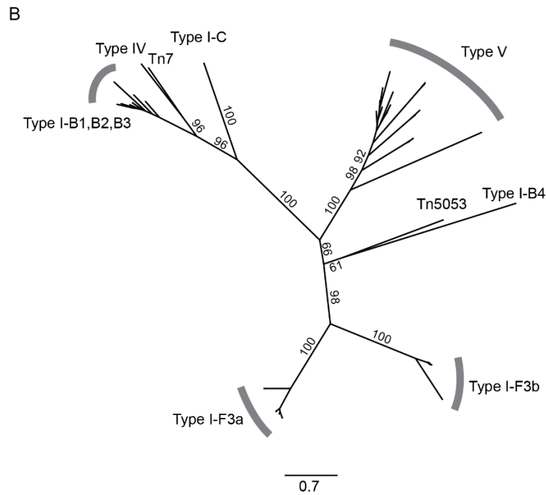
Supplemental Figure 1. Phylogenetic tree of (A) tnsB and (B) tnsC genes from each subtype of Tn7 CAST investigated in this work, as well as from Tn7 and Tn5053. Values at branch points are bootstrap support percentages.
