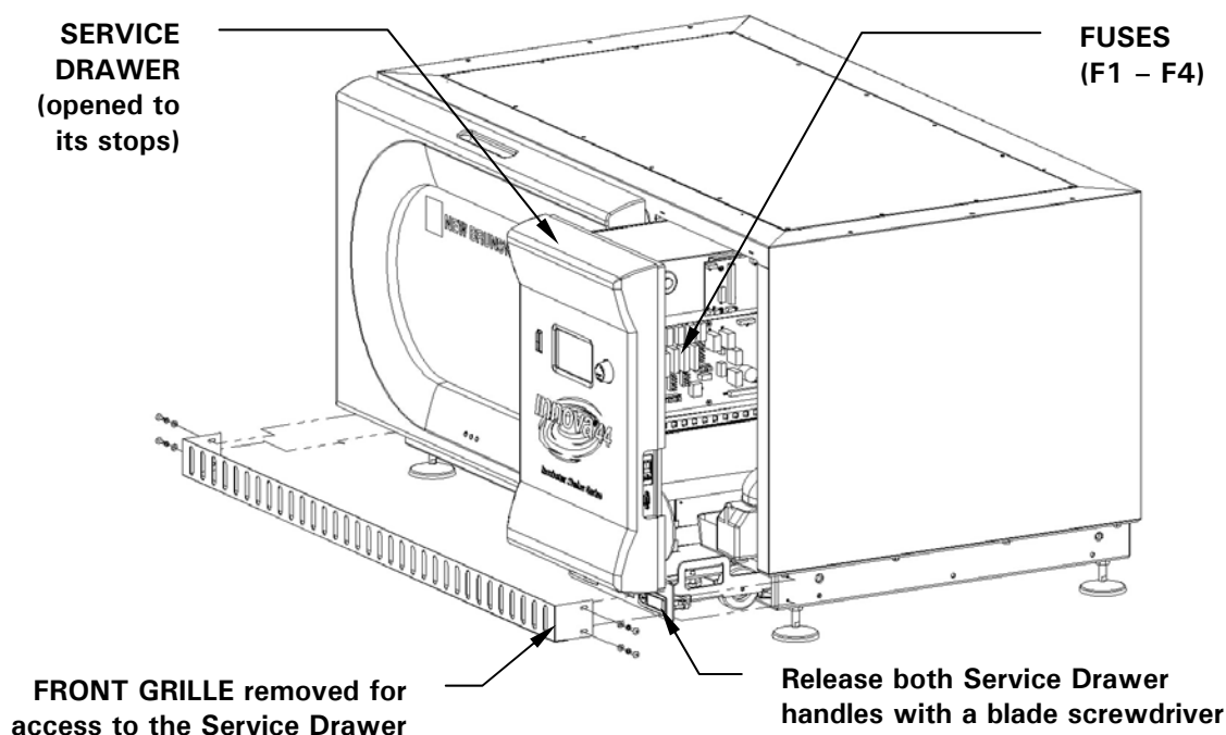
Figure 28: Fuse Replacement
