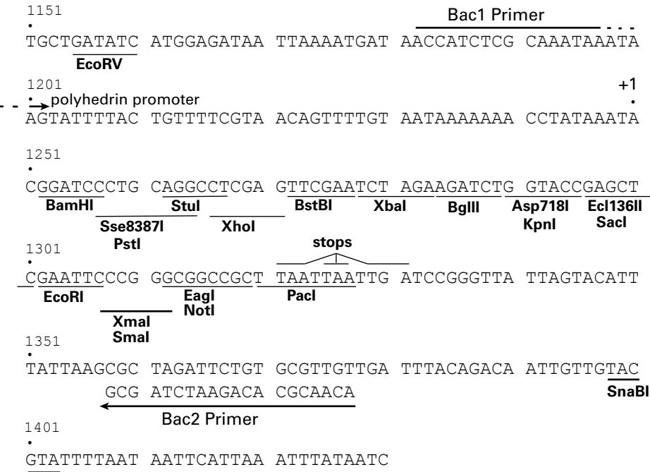
Figure 3. Map of pBacPAK8 Transfer Vector.
