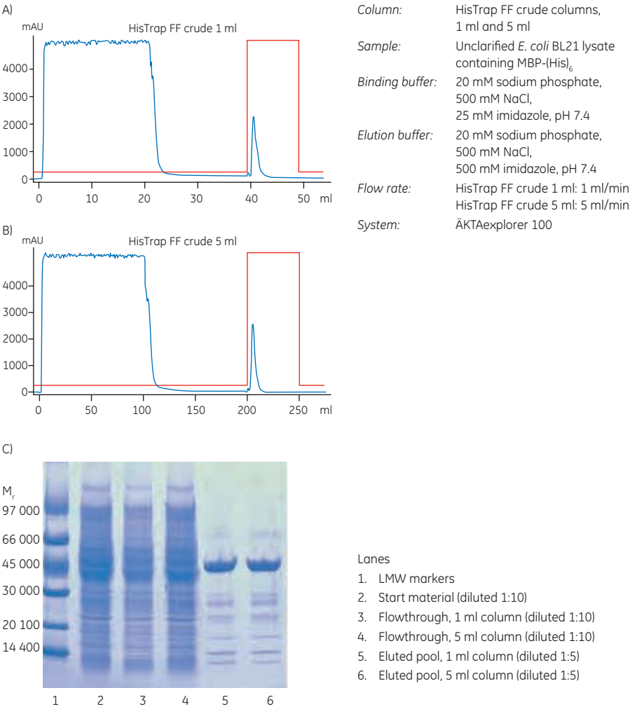
Fig 3.22. Scale-up from (A) 1 ml to (B) 5 ml HisTrap FF crude columns. Recovery of protein was 6.3 and 35.2 mg for the 1 ml and 5 ml columns, respectively. (C) SDS-PAGE under nonreducing conditions (ExcelGel SDS Gradient 8–18) confirms that scaling up from the 1 ml to the 5 ml column does not significantly affect the purification result.
