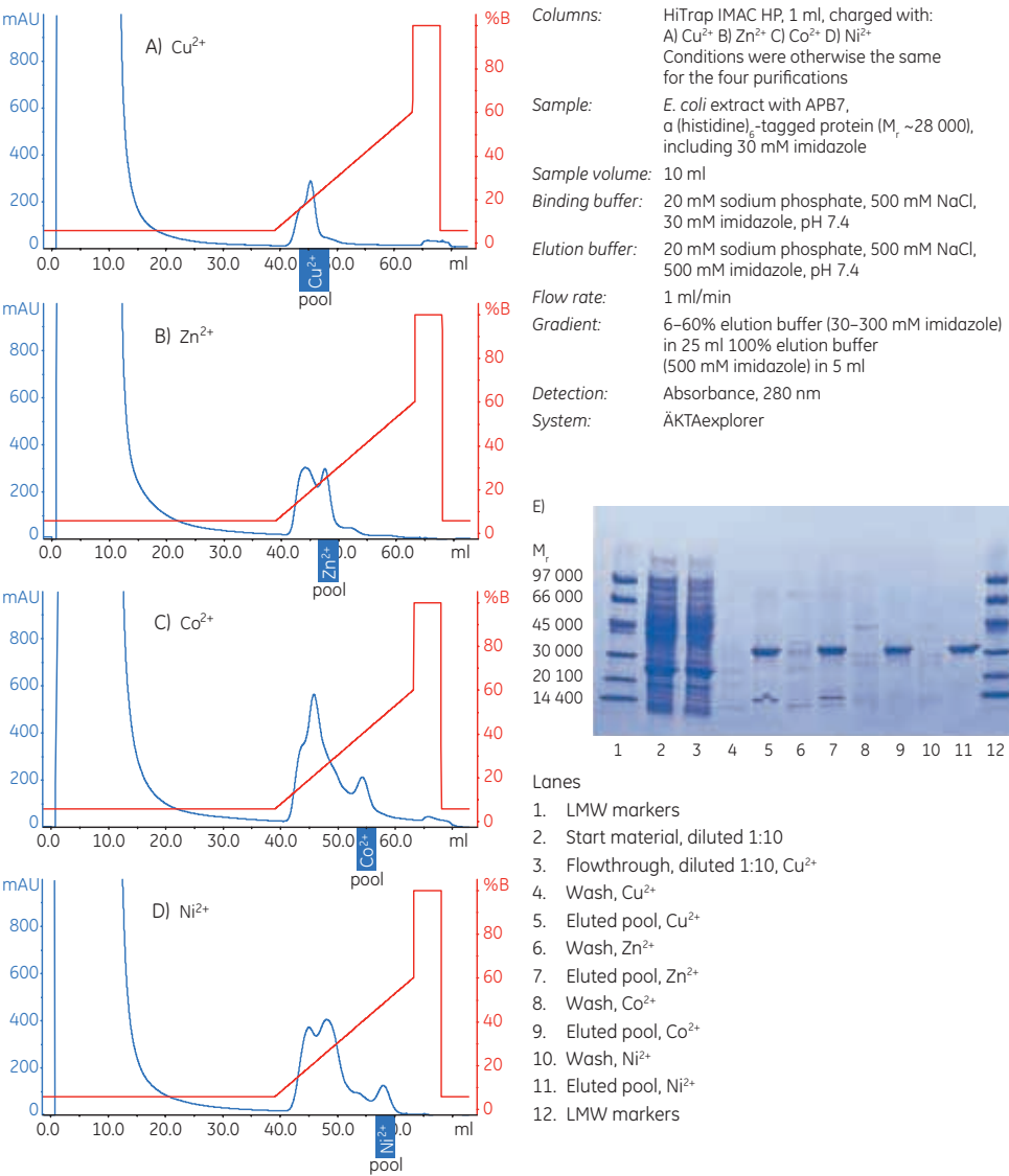
Fig 4.4. Purification of APB7, a (histidine) 6 -tagged protein expressed in E. coli BL-21 on four different HiTrap IMAC HP 1 ml columns charged separately with metal ions. (A) Cu 2+ , (B) Zn 2+ , (C) Co 2+ , or (D) Ni 2+ . Pools selected after SDS-PAGE of individual 1 ml fractions (not shown) are indicated. (E) SDS-PAGE analysis: reducing conditions on ExcelGel SDS Gradient 8–18; Coomassie staining.
