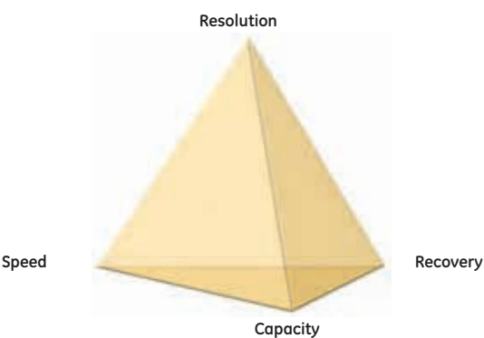
Fig 9.2. Every chromatographic technique offers a balance between resolution, capacity, speed, and recovery.
