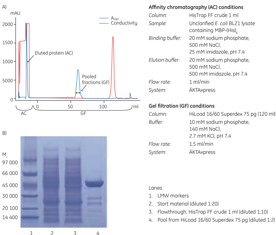
Fig 3.23. (A) Automated two-step purification of MBP-(His) 6 from an unclarified lysate of E. coli using HisTrap FF crude and HiLoad 16/60 Superdex 75 pg on ÄKTExpress. (B) SDS-PAGE was performed under nonreducing conditions on ExcelGel SDS Gradient 8–18.
