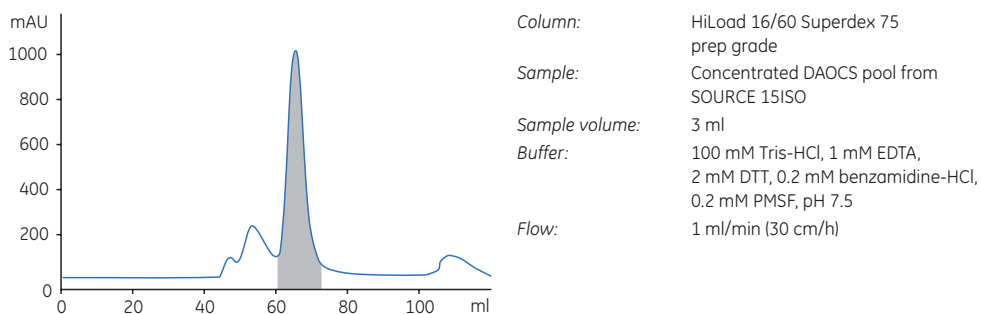
Fig 9.6. Polishing step using gel filtration. The elution position of DAOCS is shaded.
