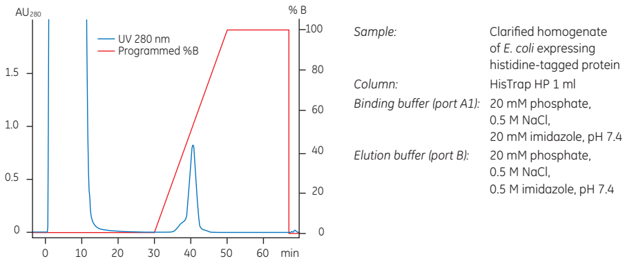
Fig 3.18. Typical result from gradient elution of a histidine-tagged protein.
