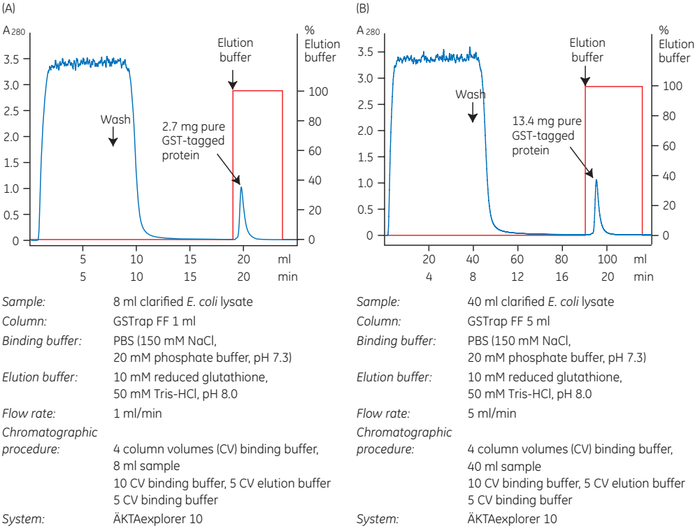
Fig 5.11. Purification of a GST-tagged protein on GSTrap FF 1 ml and 5 ml columns in combination with ÄKTAexplorer 10. Cytoplasmic extract (8 and 40 ml) from E. coli expressing a GST-tagged protein were applied to GSTrap FF 1 ml (A) and GSTrap FF 5 ml (B), respectively.
