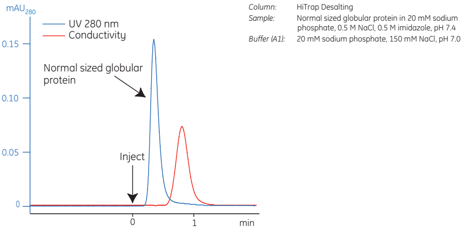
Fig 11.13. Typical desalting of a normal sized globular protein using a chromatography system.
