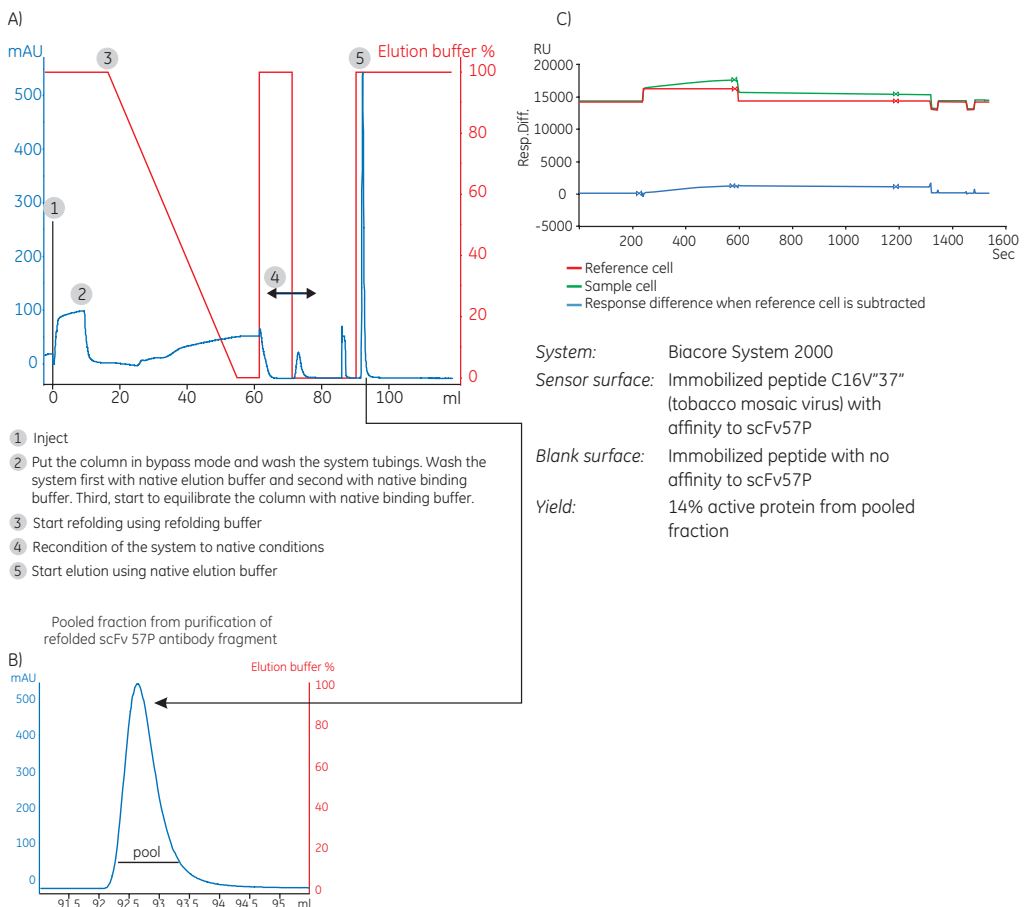
Fig 3.12 (A). On-column folding and purification. (B) Enlarged figure of pooled fraction from purification of refolded scFv 57P antibody fragment. (C) Sensogram of the interaction between immobilized peptide and refolded protein.
