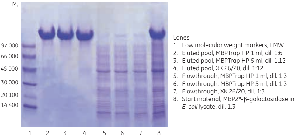
Fig 6.8. SDS-PAGE analysis (reduced conditions) of the scale-up study.
