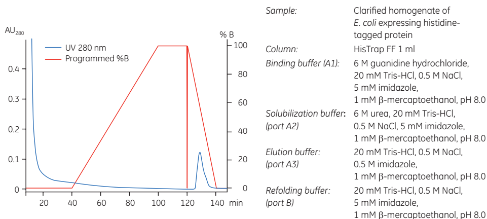
Fig 10.3. On-column refolding of a histidine-tagged protein.
