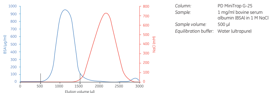
Fig 11.7. Removal of NaCl from BSA using the gravity protocol. The protein recovery was 95%.
