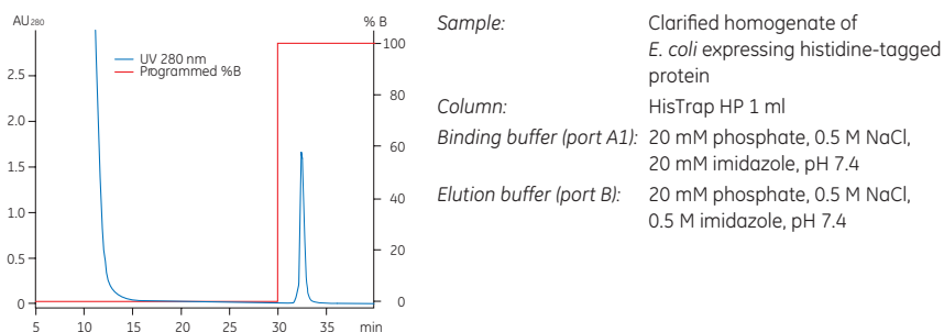
Fig 3.16. Typical result from step elution of a histidine-tagged protein.
