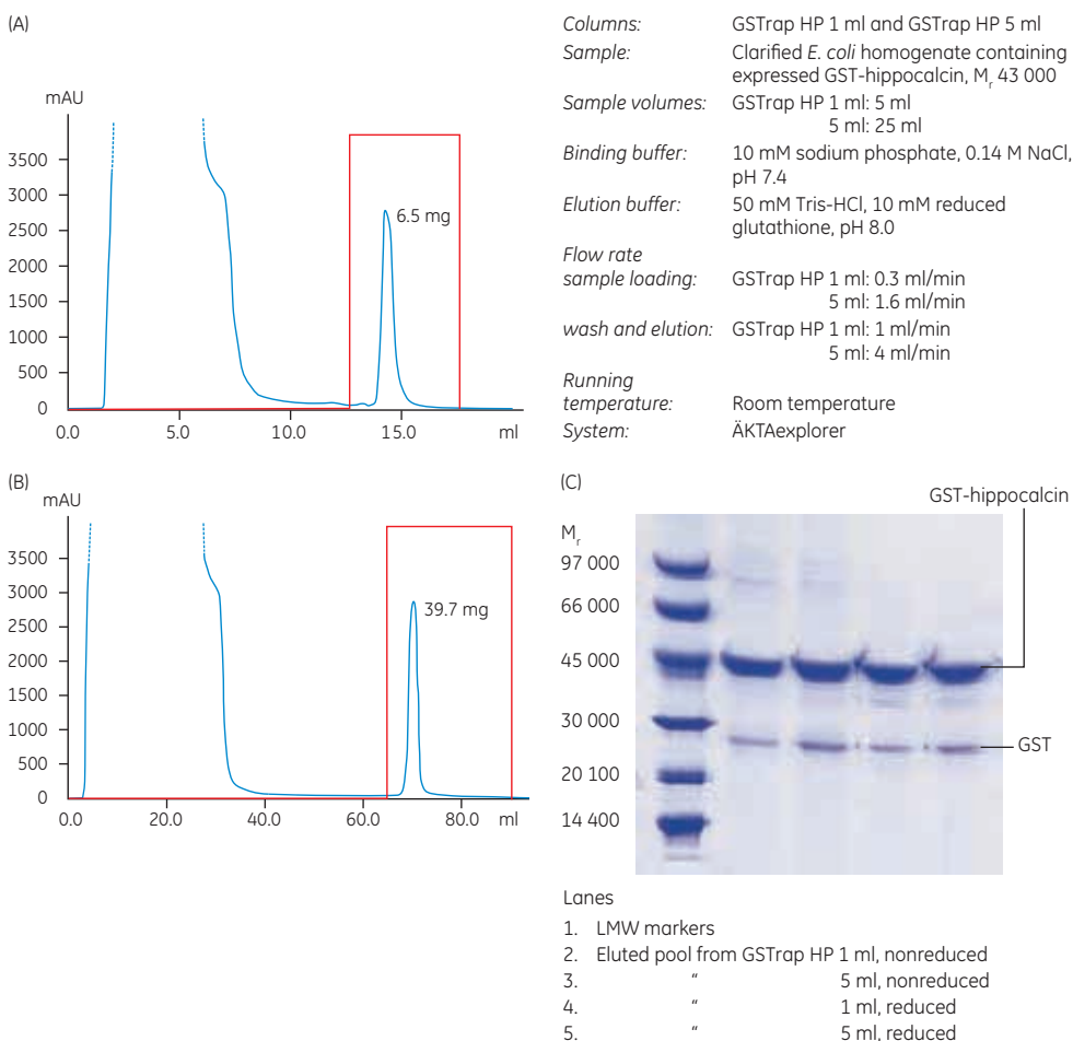
Fig 5.10. Scale-up from (A) GSTrap HP 1 ml to (B) GSTrap HP 5 ml. (C) Coomassie-stained reduced and nonreduced SDS-PAGE (ExcelGel SDS Gradient 8–18) of fractions from purification shown in Fig 5.10A–B.
