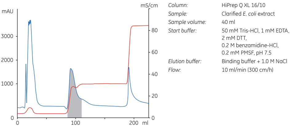
Fig 9.4. Capture using IEX. The elution position of DAOCS is shaded.
