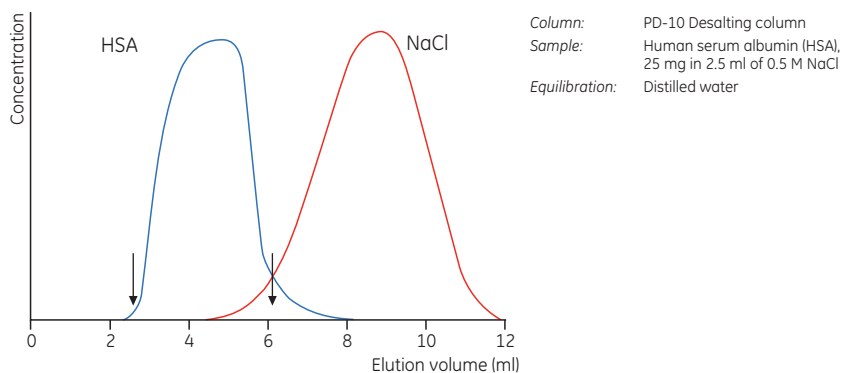
Fig 11.8. Removal of NaCl from albumin solution. A PD-10 Desalting column was equilibrated with distilled water. A total of 23.8 mg albumin was recovered in 3.5 ml eluent corresponding to a yield of 95.3% (between arrows).
