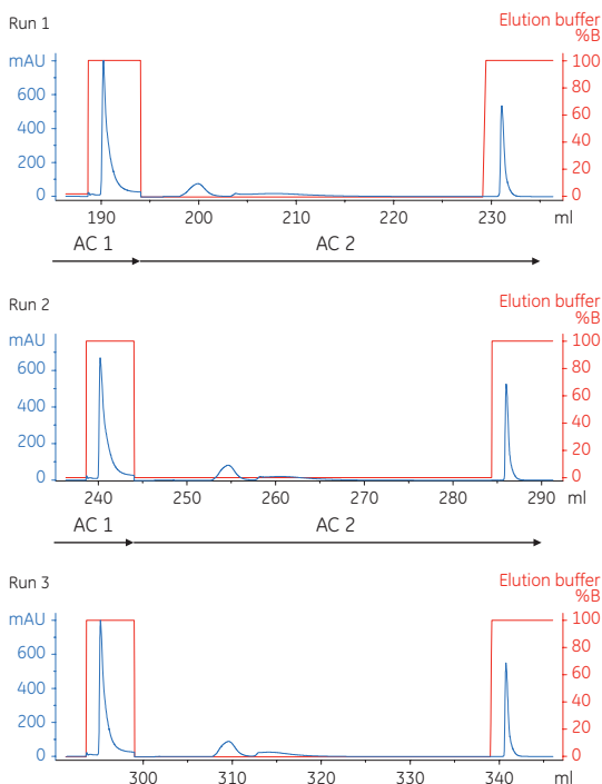
Fig 7.5. Automated purification of dual-tagged fluorescent protein (His) 6 -mCherry-Strep-tag II using two-step affinity on StrepTrap HP 1 ml (AC 1, eluted peak shown) and HisTrap HP 1 ml (AC 2, whole run shown).
