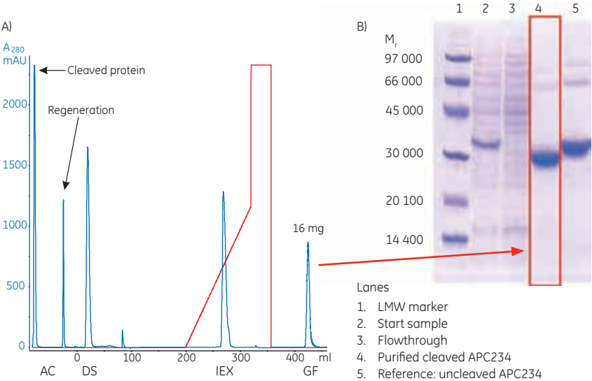
Fig 3.36. (A) Four-step protocol for purification of (histidine) 6 -tagged protein cleaved with AcTEV protease. (B) SDS-PAGE analysis. The gel was stained with Coomassie.
