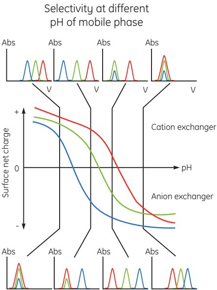
Fig A11.3. Effect of pH on protein elution patterns. V = volume.
