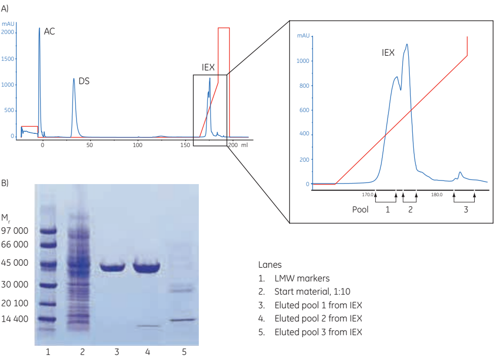
Fig 4.6. (A) AC-DS-IEX with an enlargement of the IEX peaks and the collected pools to the right. Yield: 9.4 mg in pools 1 + 2. (B) SDS-PAGE of eluted pools from IEX. The gel was stained with Coomassie.
