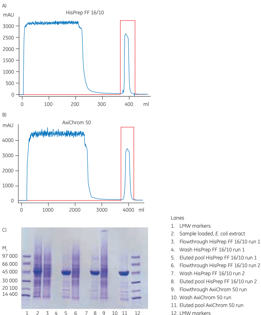
Fig 3.14. Scale-up from (A) HisPrep FF 16/10 (20 ml) to (B) AxiChrom 50 (210 ml) column. ÄKTAexplorer 100 was used for the purification runs on HisPrep FF 16/10 columns and ÄKTA Pilot was used for AxiChrom 50 purification. All systems were controlled by UNICORN software. Note that only the chromatogram for run 1 on HisPrep FF 16/10 is presented. (C) SDS-PAGE of various fractions from both purifications.
