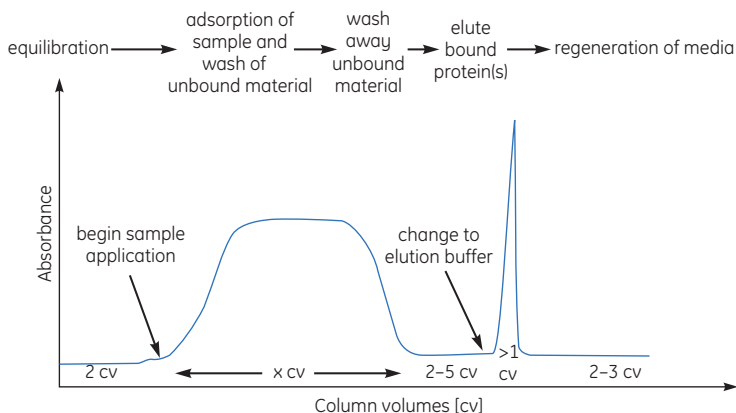
Fig A11.1. Typical affinity purification.
