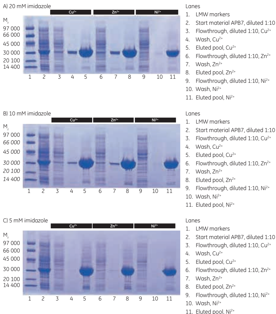
Fig 4.3. SDS-PAGE analyses (reducing conditions) of fractions from the purification of APB7 using IMAC Sepharose 6 Fast Flow, prepacked in HiTrap IMAC FF 1 ml columns, charged with either \text{Cu}^{2+} , \text{Zn}^{2+} , or \text{Ni}^{2+} , and with (A) 20 mM imidazole in the sample, (B) 10 mM imidazole in the sample, or (C) 5 mM imidazole in the sample. The gels were stained with Coomassie.
