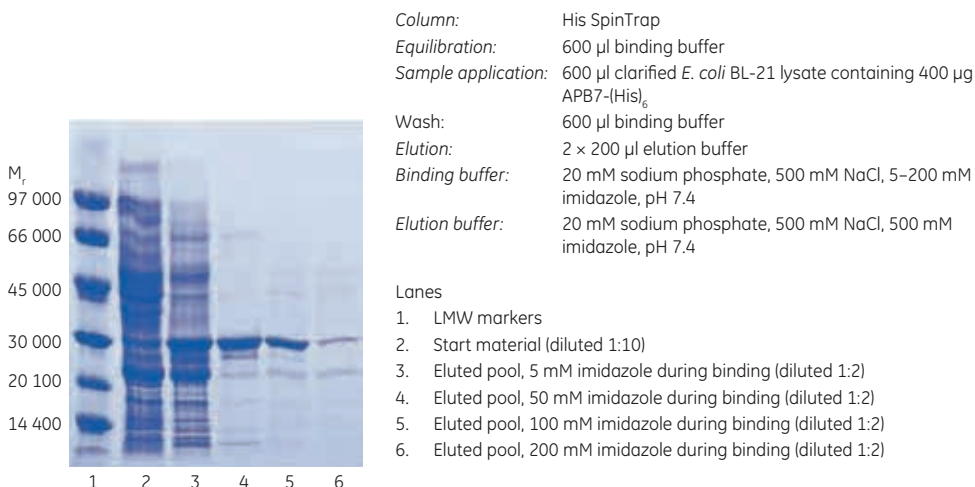
Fig 4.2. SDS-PAGE under reducing conditions (ExcelGel SDS Gradient 8–18) of histidine-tagged APB7 protein. The imidazole concentration during binding affects the final purity and yield (compare lanes 3, 4, 5, and 6).
