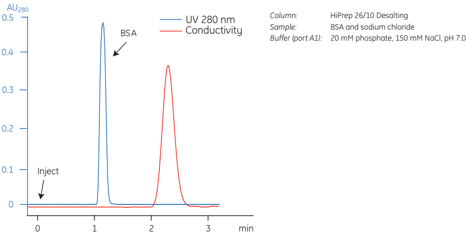
Fig 11.15. A typical desalting of BSA using a chromatography system.
