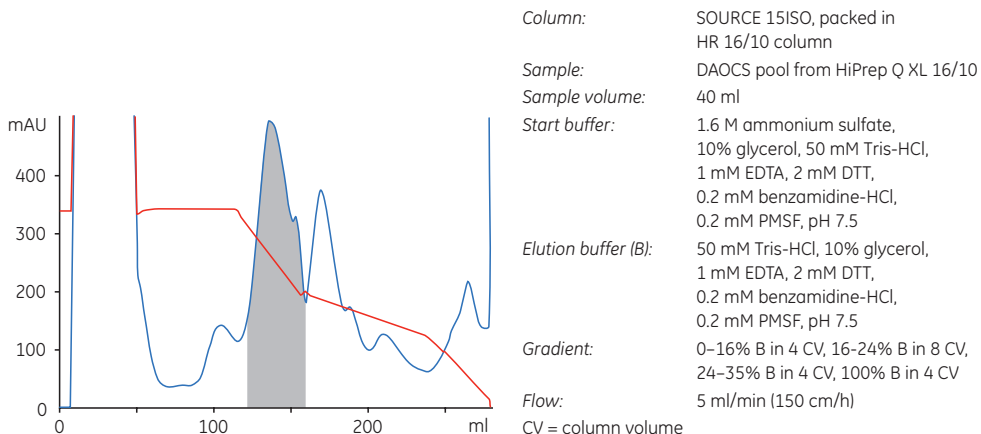
Fig 9.5. Intermediate purification using HIC. The elution position of DAOCS is shaded.
