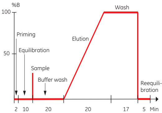
Fig 3.17. Theoretical gradient (programmed %B) in His Tag Purification HisTrap Application Template. Total separation time = 74 min + sample application time.
