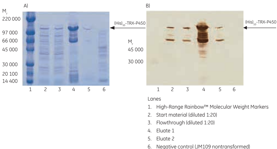
Fig 3.28. (A) SDS-PAGE and (B) Western blot of (His) 10 -TRX-P450 purified using His GraviTrap column.
