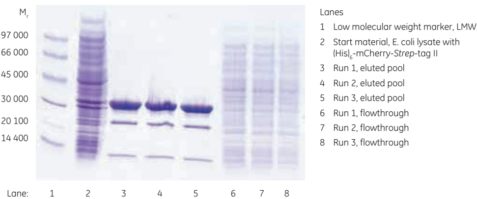
Fig 7.6. SDS-PAGE analysis (reduced conditions) of the three different automated two-step affinity purification of (His) 6 -mCherry-Strep-tag II.
