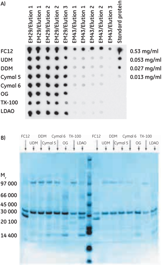
Fig 3.6. (A) Dot blot of membrane proteins EM29 and EM43 purified on His MultiTrap FF in the presence of different detergents. Repeats of eluates 1 and 2 shown in the dot blot are two independent extractions and purifications. (B) SDS-PAGE (Coomassie staining) of EM29 purifications (elutions 1 and 2 in the blot) with eight different detergents on His MultiTrap FF. Data kindly provided by S. Eshagi, V. Lieu, P. Nordlund, Dept. of Medical Biochemistry and Biophysics, Karolinska Institute, Stockholm, Sweden.
