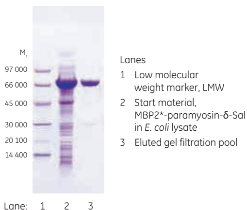
Fig 6.4. SDS-PAGE analysis (reduced conditions) of the purification of MBP2*-paramyosin- \delta -Sal.
