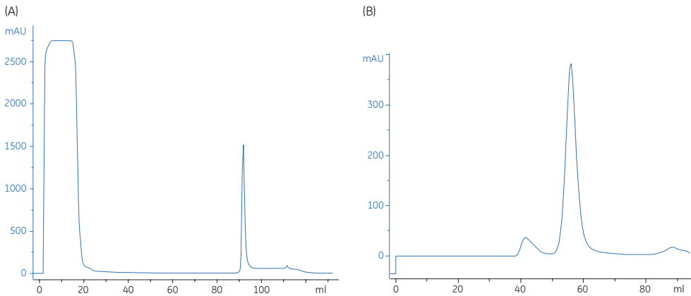
Fig 6.5. Purification of MCAD on (A) MBPTrap HP followed by (B) Superdex 200 pg.
