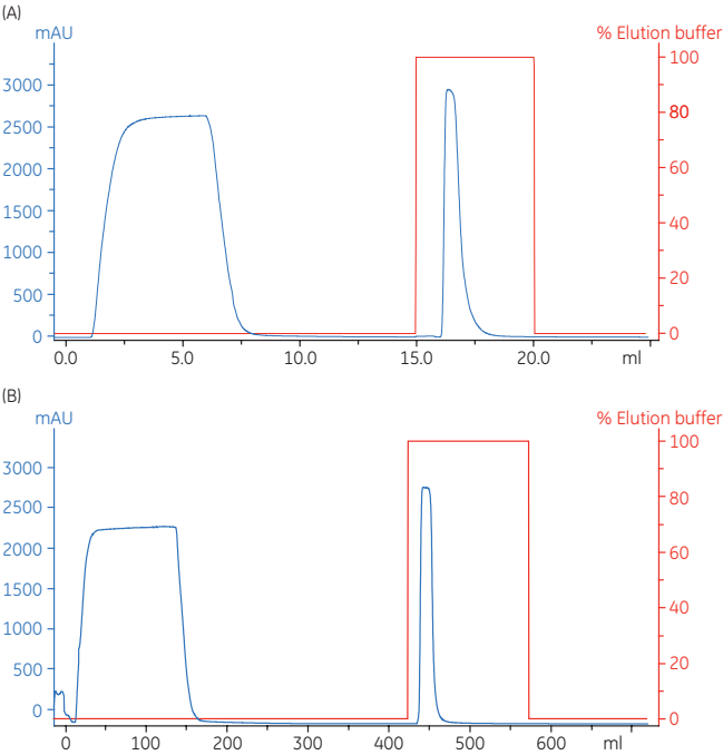
Fig 6.7. Scale-up of MBP2*-β-galactosidase purification, (A) MBPTrap HP 1 ml (B) Dextrin Sepharose High Performance XK 26/20, 29 ml. Chromatogram for MBPTrap 5 ml column not shown.
