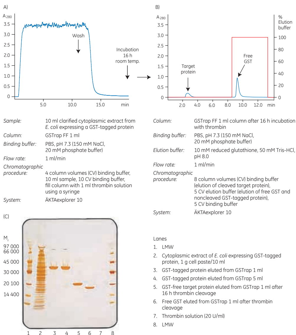
Fig 5.24. On-column thrombin cleavage of a GST-tagged protein. (A) Equilibration, sample application, and washing of a GST-tagged protein on GSTrap FF 1 ml were performed using ÄKTAexplorer 10. After washing, the column was filled by syringe with 1 ml of thrombin (20 U/ml) and incubated for 16 h at room temperature. (B) GST-free target protein was eluted using PBS, pH 7.3. GST was eluted using 10 mM reduced glutathione. (C) SDS-PAGE followed by silver staining. The GST-free target protein fraction also contained a small amount of thrombin not detectable by SDS-PAGE (lane 6). The thrombin can be removed using a HiTrap Benzamidine FF (high sub) column.
