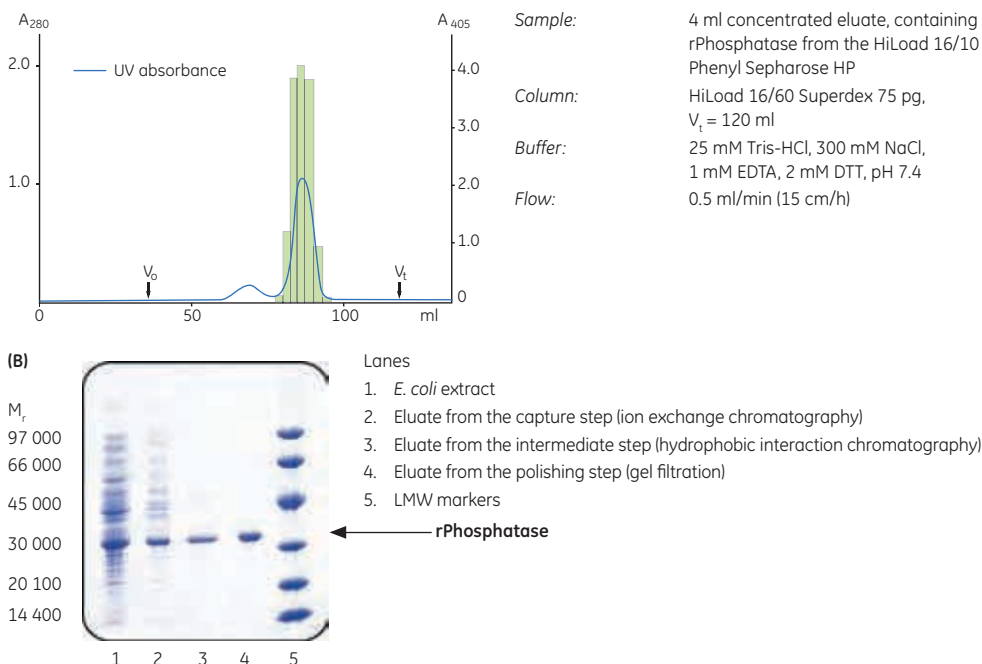
Fig 9.9. (A) Polishing step using gel filtration. The phosphatase activity is represented by the green bars (absorbance at 405 nm). (B) Purity check by SDS-PAGE. The proteins were stained with Coomassie Brilliant Blue.
