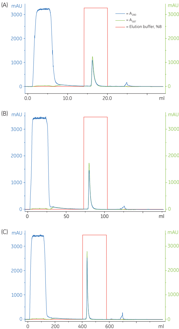
Fig 7.4. Scaling up the purification of (His) 6 -mCherry-Strep-tag II, (A) StrepTrap HP 1 ml, (B) StrepTrap HP 5 ml, (C) StrepTactin Sepharose High Performance XK 26/20 with 5.5 ml bed height, 29 ml.
