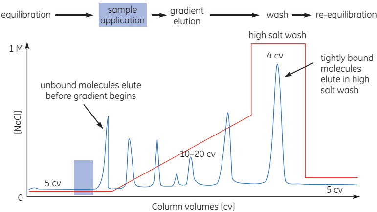
Fig A11.2. Typical IEX gradient elution. Blue line = absorbance; red line = conductivity (salt concentration).
