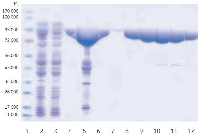
Fig 6.5. Purification of MCAD on (A) MBPTrap HP followed by (B) Superdex 200 pg.
