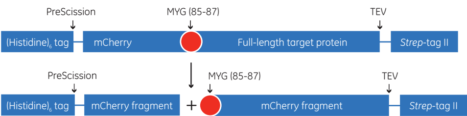
Fig 7.7. Cleavage of (His) 6 -mCherry-Strep-tag II between F(84) and the MYG chromophore yields an N-terminal fragment of M_r 9558 and a C-terminal fragment of M_r 20 741.
