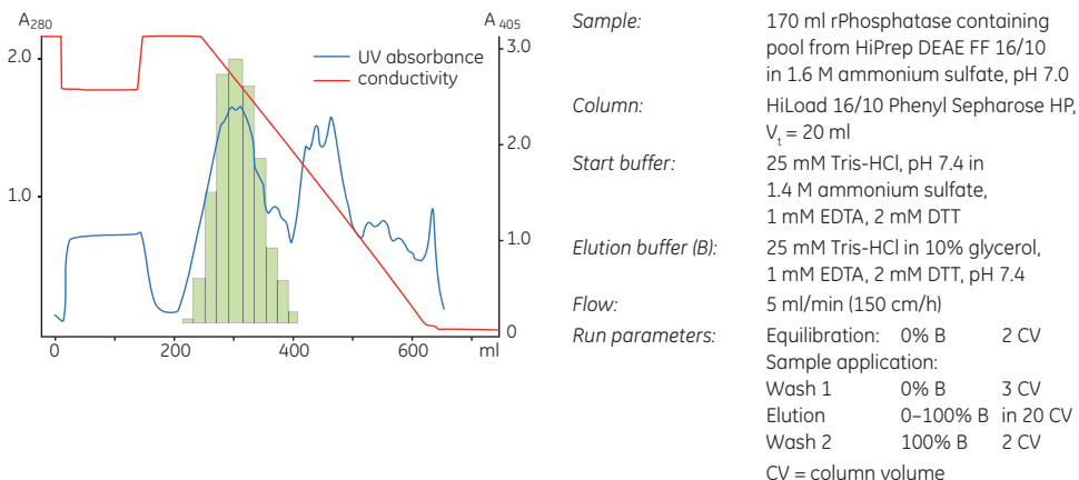
Fig 9.8. Intermediate purification step using hydrophobic interaction. The phosphatase activity is represented by the green bars (absorbance at 405 nm).
