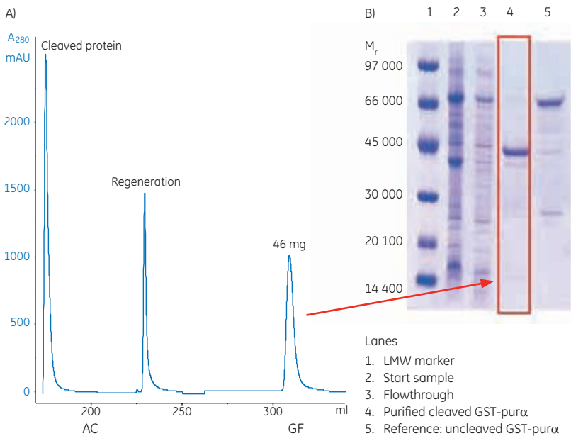
Fig 5.22. (A) Two-step protocol for automatic GST-tagged protein cleavage with PreScission Protease and purification. (B) Analysis of the untagged target protein after purification and GST-tagged cleavage on SDS-PAGE and Coomassie staining.
