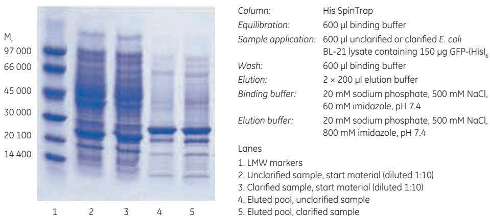
Fig 3.9. SDS-PAGE (ExcelGel™ SDS Gradient 8–18) under reducing conditions of unclarified and clarified E. coli lysate containing GFP-(His) 6 . Similar purity and recovery were observed for both unclarified and clarified sample.
