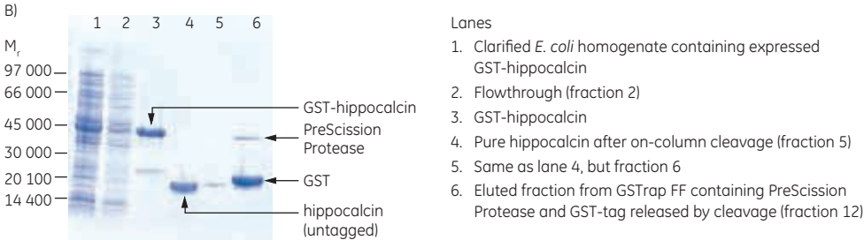
Fig 5.21. Purification of human hippocalcin-GST-tagged protein with on-column cleavage and post-cleavage removal of PreScission Protease using GSTrap FF columns. A) Chromatogram showing purification of hippocalcin. B) SDS-PAGE analysis of various sample processing steps. ExcelGel SDS Gradient, 8–18%, Coomassie blue staining.
