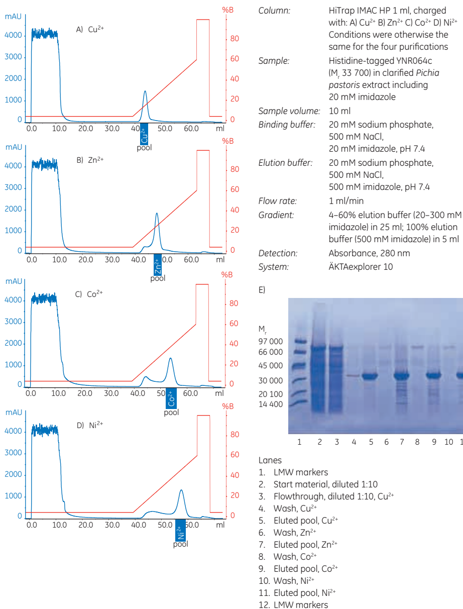
Fig 3.34. Purification of (histidine) 6 -tagged YNR064c expressed in Pichia pastoris on four different HiTrap IMAC HP 1 ml columns charged separately with metal ions (A) Cu 2+ , (B) Zn 2+ , (C) Co 2+ , or (D) Ni 2+ . Pools selected after SDS-PAGE of individual 1 ml fractions (not shown) are indicated. (E) SDS-PAGE analysis: reducing conditions on ExcelGel SDS Gradient 8–18; Coomassie staining.
