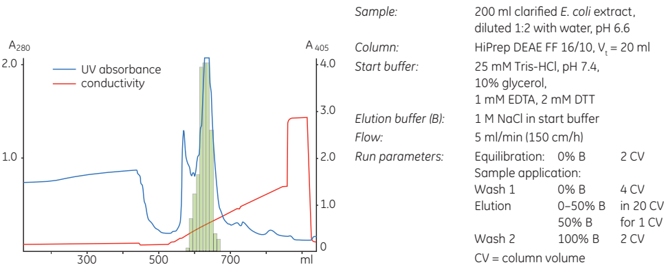
Fig 9.7. Capture step using ion exchange. The phosphatase activity is represented by the green bars (absorbance at 405 nm).
