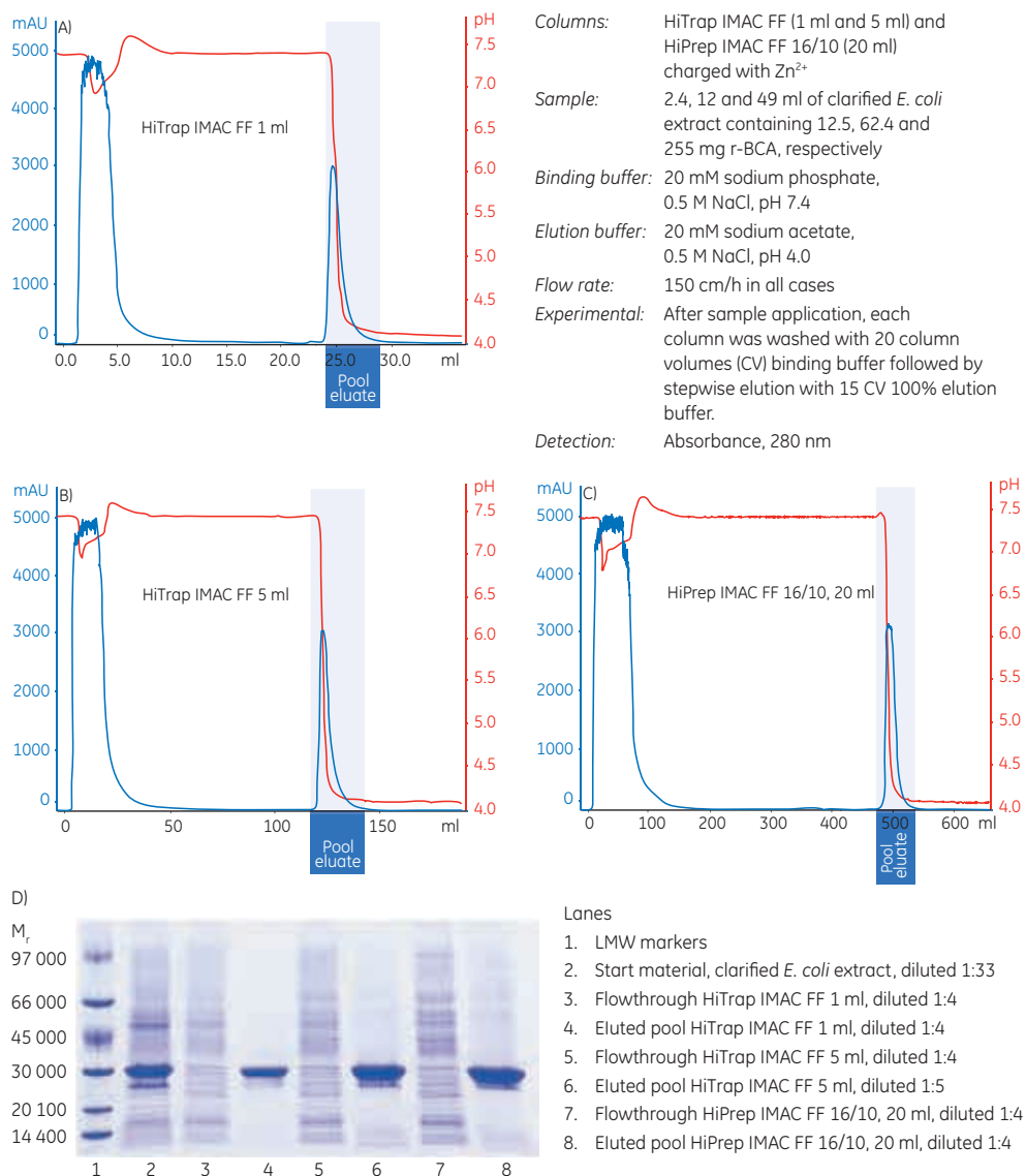
Fig 3.35. Chromatograms showing scale-up of purification from (A) HiTrap IMAC FF 1 ml column to (B) HiTrap IMAC FF 5 ml column and (C) HiPrep IMAC FF 16/10 20 ml column. Sample was 2.4, 12, and 49 ml of clarified extract of E. coli containing 12.5, 62.4, and 255 mg of r-BCA, respectively. The load was approximately 74% of maximum binding capacity. (D) Nonreduced SDS-PAGE analysis on ExcelGel Gradient 8-18 of the main fractions from the scale-up experiments. The gel was stained with a 1% solution of PhastGel Blue R (Coomassie).
