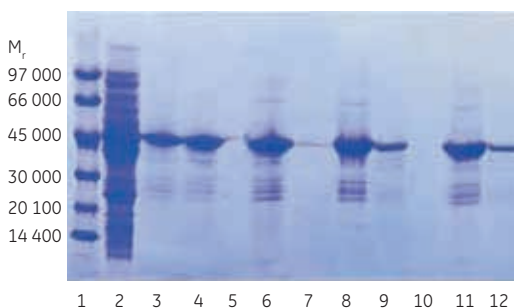
Fig 5.5. SDS-PAGE (reducing conditions, ExcelGel SDS Gradient 8–18; Coomassie staining) of collected fractions of eluted GST-hippocalcin from some of the GST MultiTrap FF filter plate wells.
