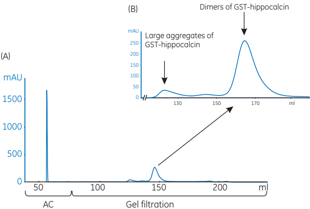
Fig 5.12. (A) Purification of GST-hippocalcin from E. coli lysate using an automated two-step purification on ÄKTAexpress. (B) Enlargement of the peak from the gel filtration step revealed large aggregates and dimers of purified GST-hippocalcin. (C) SDS-PAGE (ExcelGel SDS Gradient 8–18%) showing final purity of GST-hippocalcin (lane 4).
