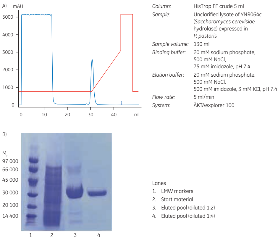
Fig 3.21. (A) Purification of an unclarified sample of histidine-tagged hydrolase from Saccharomyces cerevisiae expressed in P. pastoris on HisTrap FF crude 5 ml. (B) SDS-PAGE under nonreducing conditions (ExcelGel SDS Gradient 8–18) shows the high purity obtained of the low-level expression protein.
