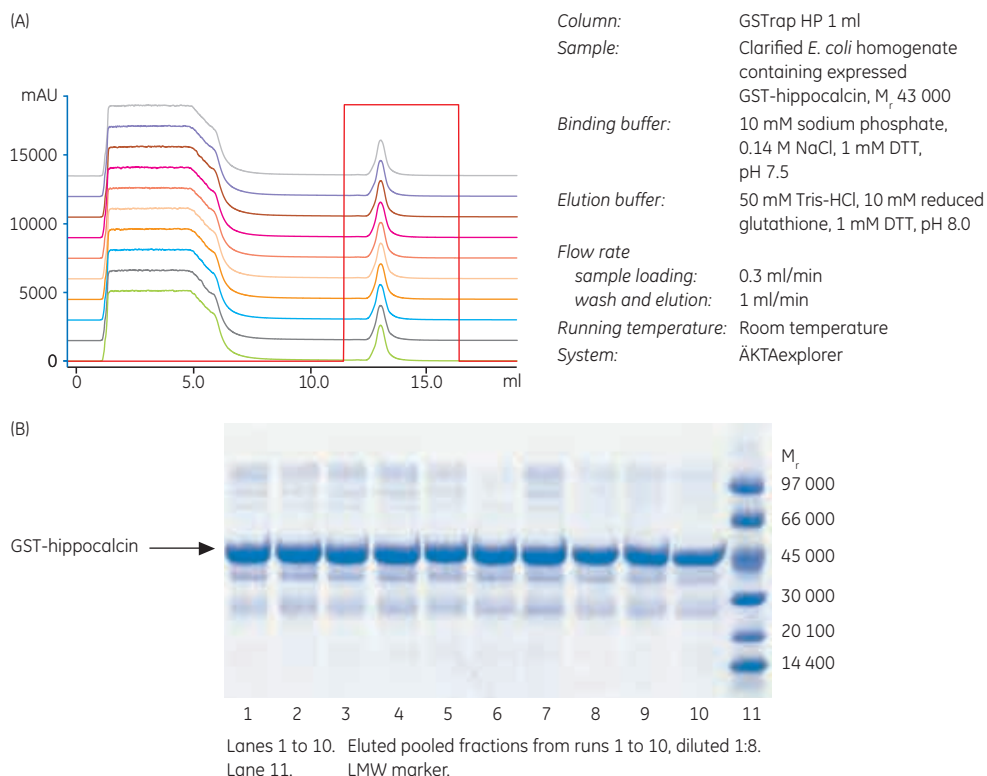
Fig 5.8. (A) Confirmation of the stability of Glutathione Sepharose High Performance prepacked in 1 ml GSTrap HP columns. Chromatographic overlay of 10 repetitive purifications. (B) Coomassie-stained nonreduced SDS-PAGE (ExcelGel SDS Gradient 8–18) of pooled fractions from repetitive purification runs shown in (A).
