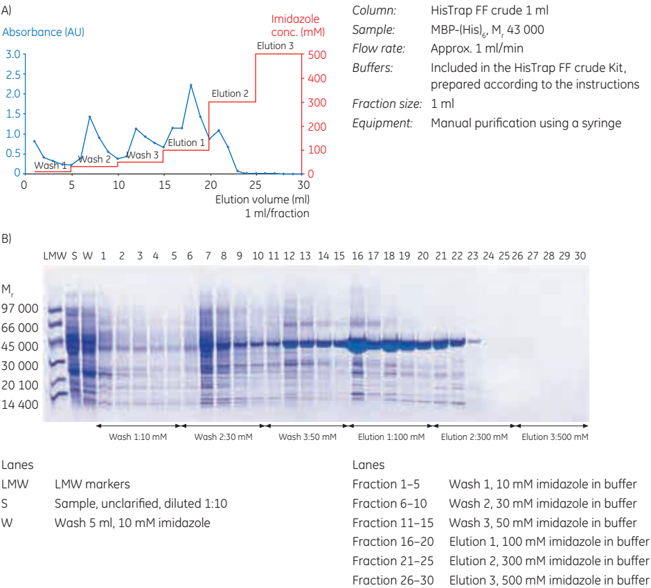
Fig 3.25. (A) Purification of MBP-(His) 6 using HisTrap FF crude Kit. (B) Native SDS-PAGE (ExcelGel 8–18) of 1 ml fractions from the purification.
