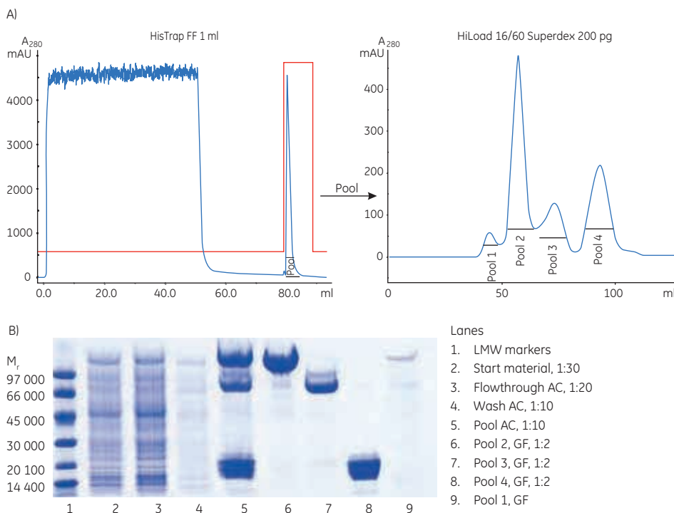
Fig 4.5. (A) Two-step purification of a high-molecular-weight (histidine) 10 -tagged protein using affinity chromatography followed by gel filtration. (B) SDS-PAGE under reducing conditions and Coomassie staining.
