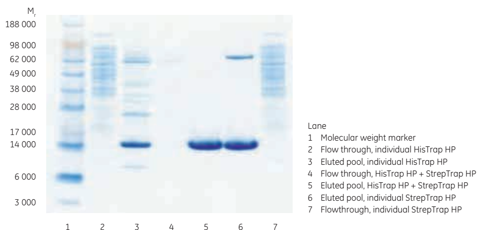
Fig 7.3. SDS-PAGE analysis (reduced conditions) comparing individual purifications on HisTrap HP 1 ml and StrepTrap HP 1 ml with a combined, two-step affinity purification on both columns. Data kindly provided by Martina Nilsson, Robert Svensson, and Erik Holmgren, Biovitrum, Stockholm, Sweden.
