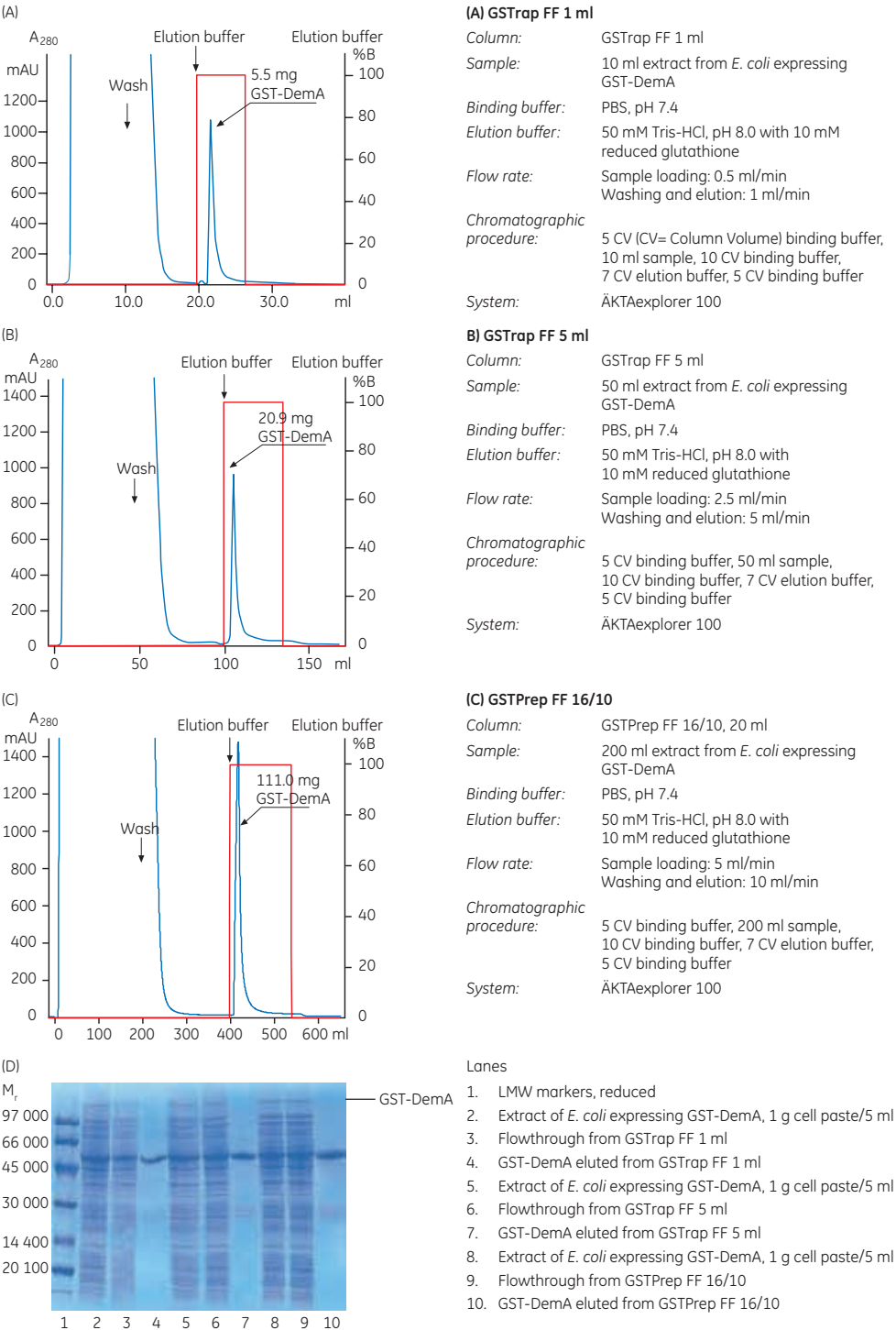
Fig 5.15. Purification and scale-up of GST-DemA on (A) GSTrap FF 1 ml, (B) GSTrap FF 5 ml, and (C) GSTPrep FF 16/10. (D) SDS-PAGE analysis of GST-DemA on ExcelGel Homogeneous 12.5% using Multiphor™ II followed by Coomassie staining. Due to the relatively slow binding kinetics of GST and rather high load, some of the applied protein was found in the flowthrough.
